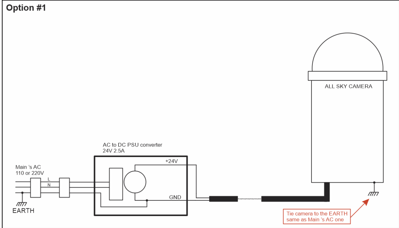
Fig. 107 System grounding scheme (Option 1)
