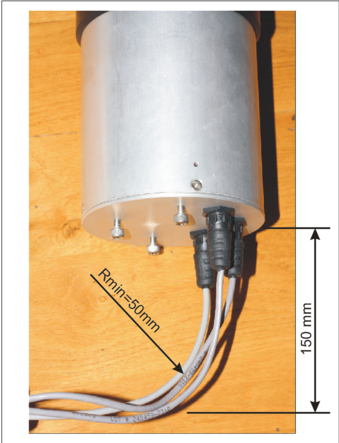
Fig. 5 Minimum cable radius curvature.
