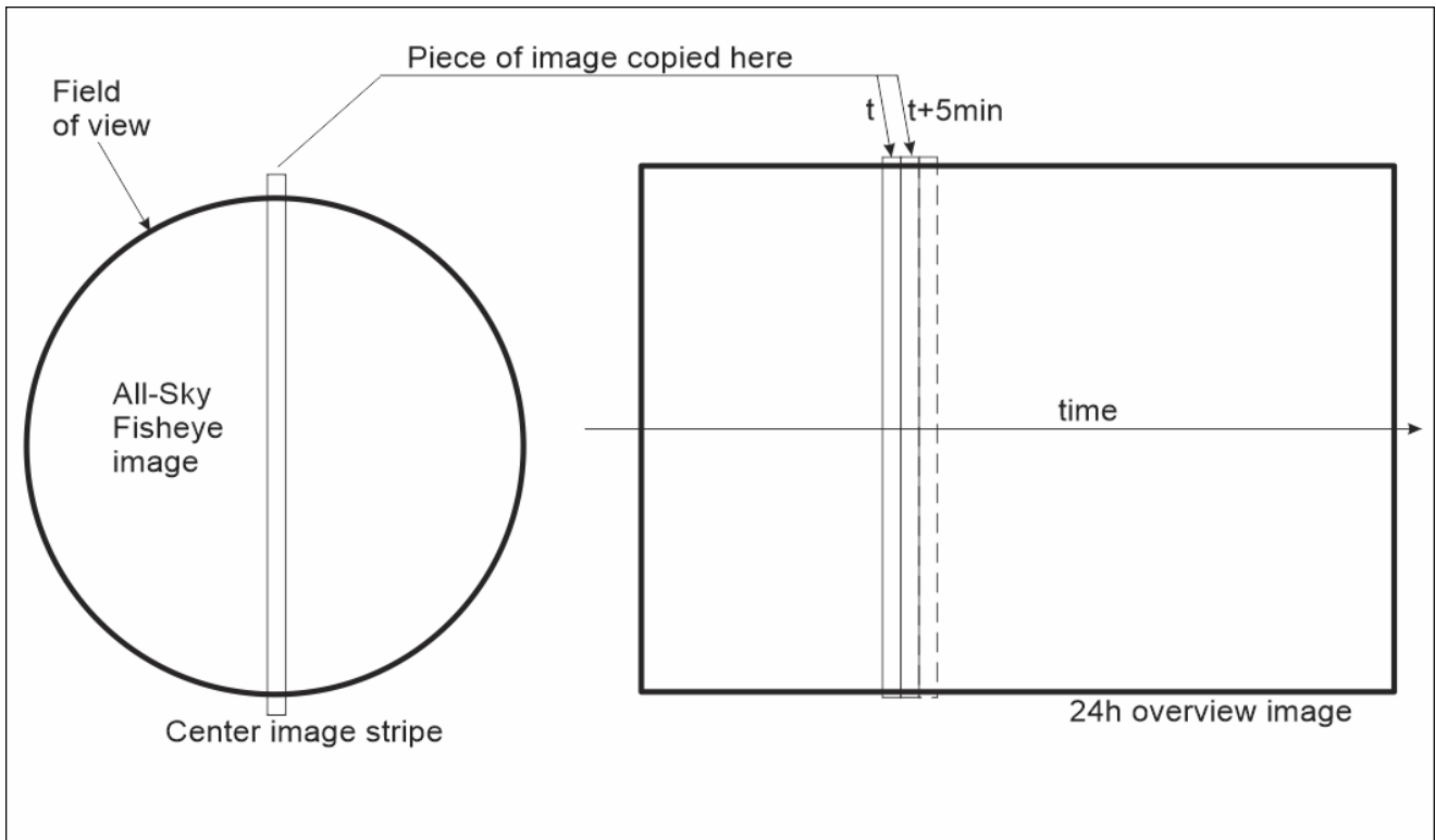
Fig. 89 : 24h image overview construction scheme
