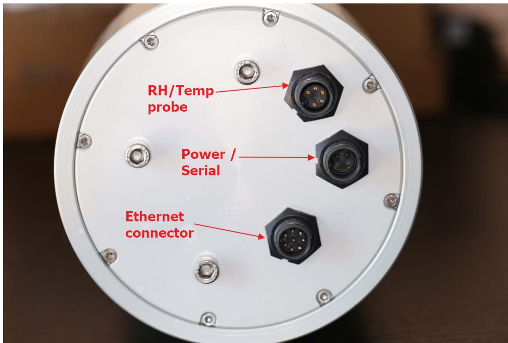
Fig. 21 : Ethernet camera backside
