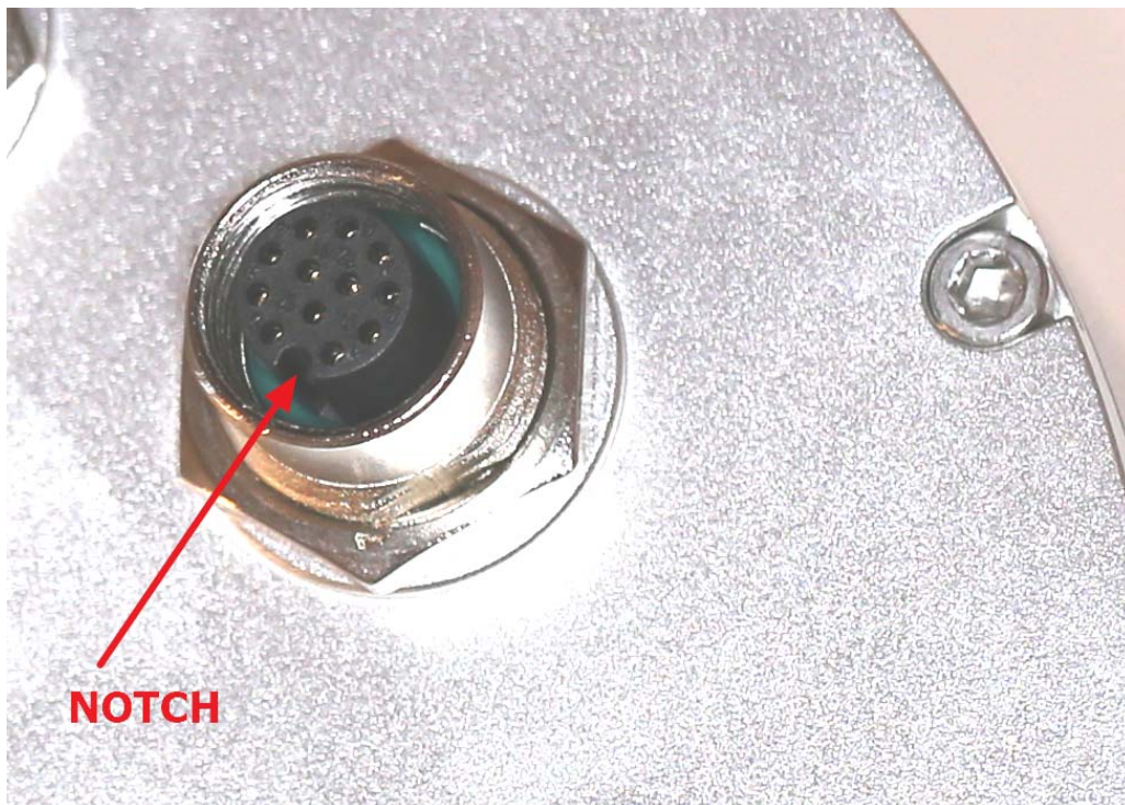
Fig. 10 All connectors have coding notch, please orientate the cable during insertion
