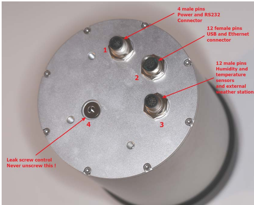
Fig. 9 New metal connectors located at camera backside
