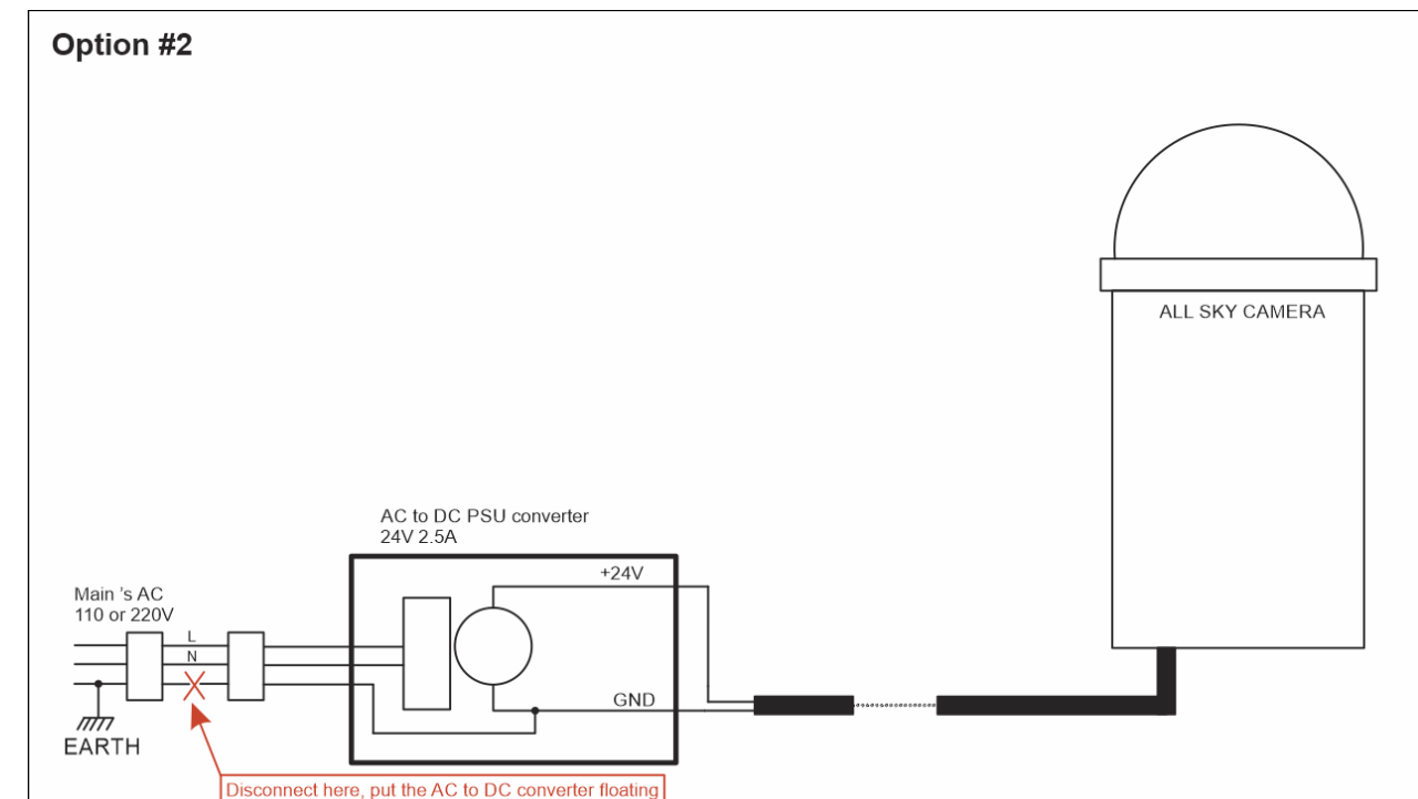
Fig. 108 System grounding scheme (Option 2)
